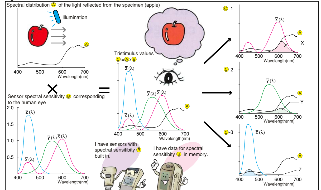
Figure 20: Determination of the tristimulus values in color measurements
